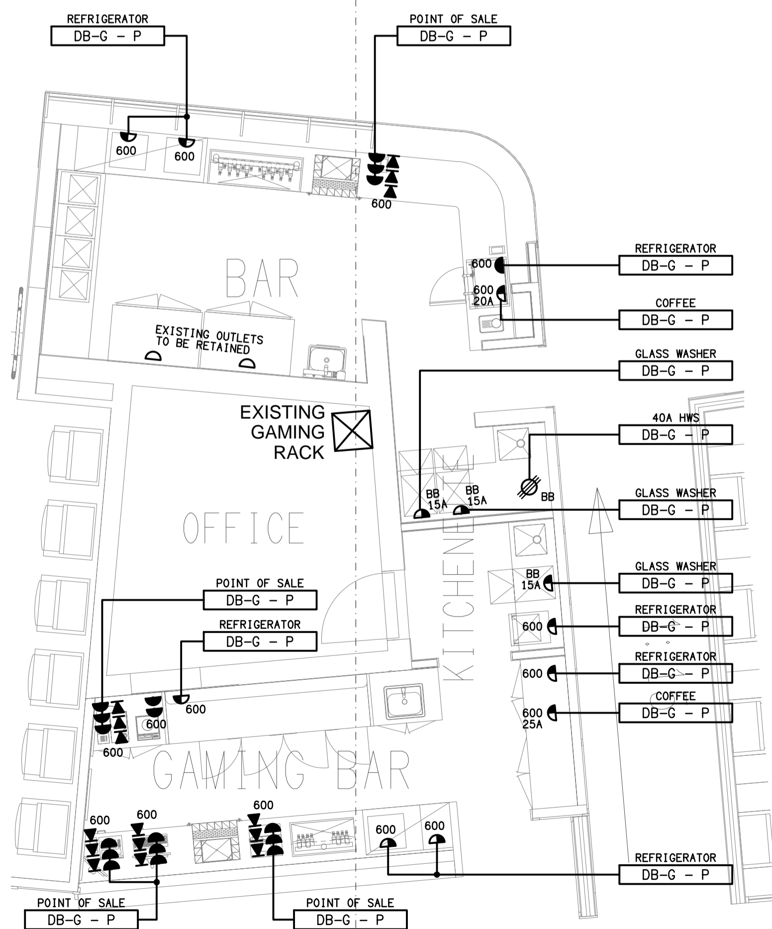
DETAIL A GAMING BAR FLOOR PLAN SCALE: 1:50
