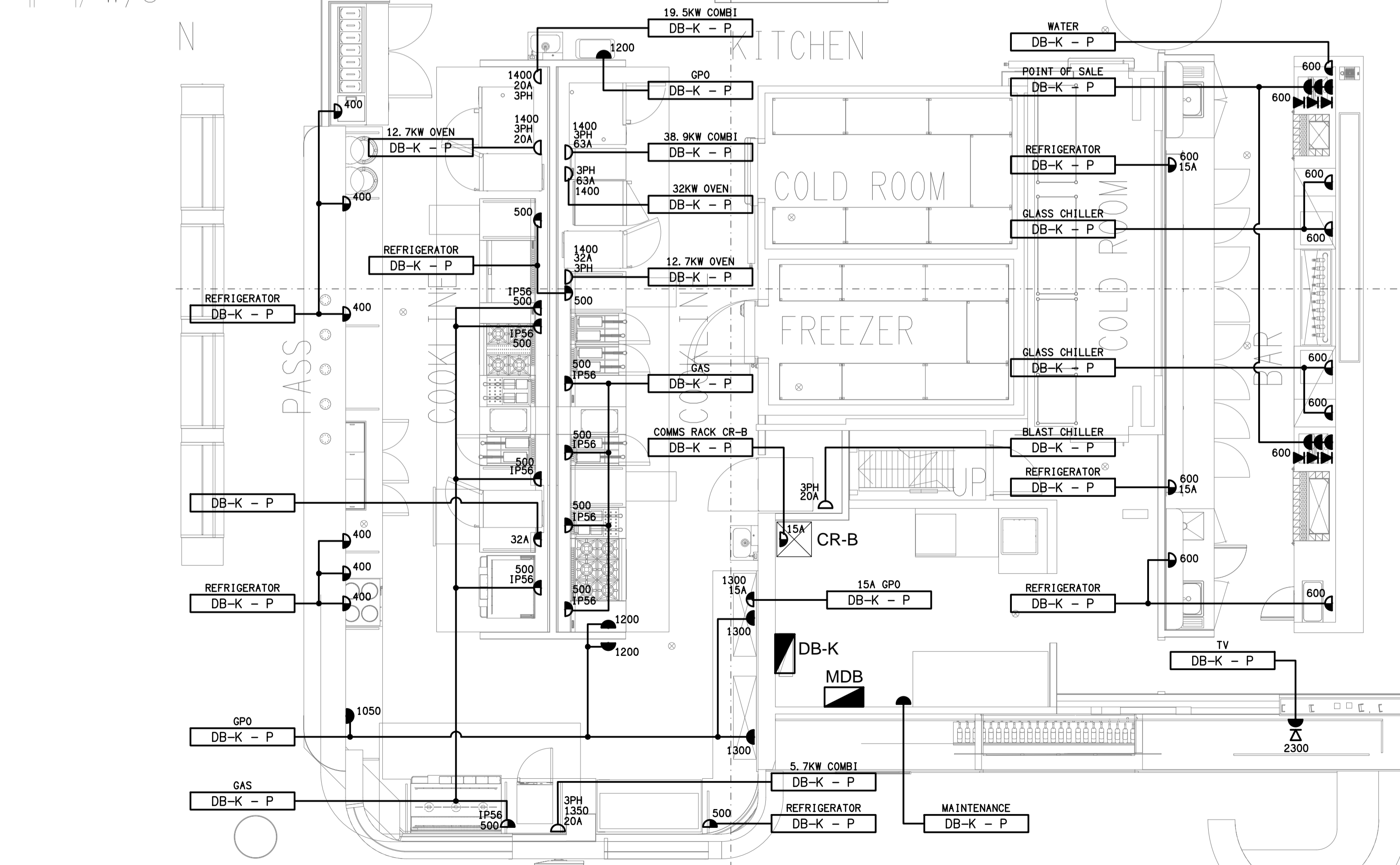
DETAIL B BISTRO KITCHEN FLOOR PLAN SCALE: 1:50
